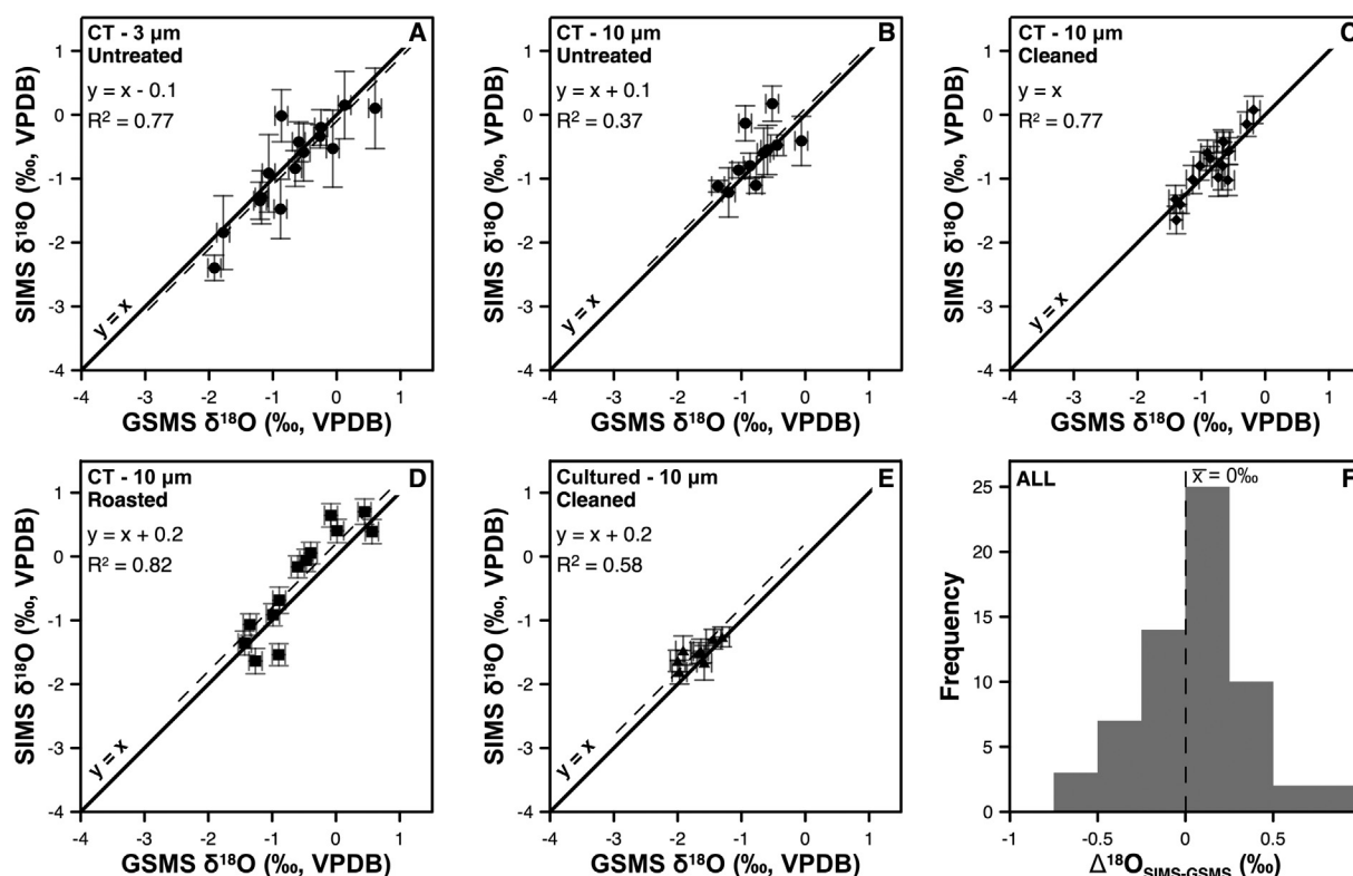
Fig. 6. Adjusted ( \pm 0.9\text{‰} ) SIMS \delta^{18}\text{O} values plotted against GSMS \delta^{18}\text{O} values from the same chamber of O. universa shells. Theoretical 1-to-1 line (solid bold line) denotes no SIMS-GSMS \delta^{18}\text{O} difference. Linear regression with slope = 1 (dashed lines) fit to data. A. Untreated core-top shells (3- \mu\text{m} SIMS analyses), B. untreated core-top shells (10- \mu\text{m} SIMS analyses), C. cleaned core-top shells (10- \mu\text{m} SIMS analyses), D. roasted core-top shells (10- \mu\text{m} SIMS analyses), and E. cleaned shells from culture experiment (10- \mu\text{m} SIMS analyses). All SIMS data shown are average chamber values, and have been adjusted (see Section 3.2). Error bars are GSMS analytical precision ( \pm 2 SD, horizontal) and propagated error from SIMS measurements ( \pm 2 SD, vertical). F. Histogram of adjusted \Delta^{18}\text{O}_{\text{SIMS-GSMS}} values for the paired datasets in A-E. Average adjusted \Delta^{18}\text{O}_{\text{SIMS-GSMS}} value (dashed vertical line).
