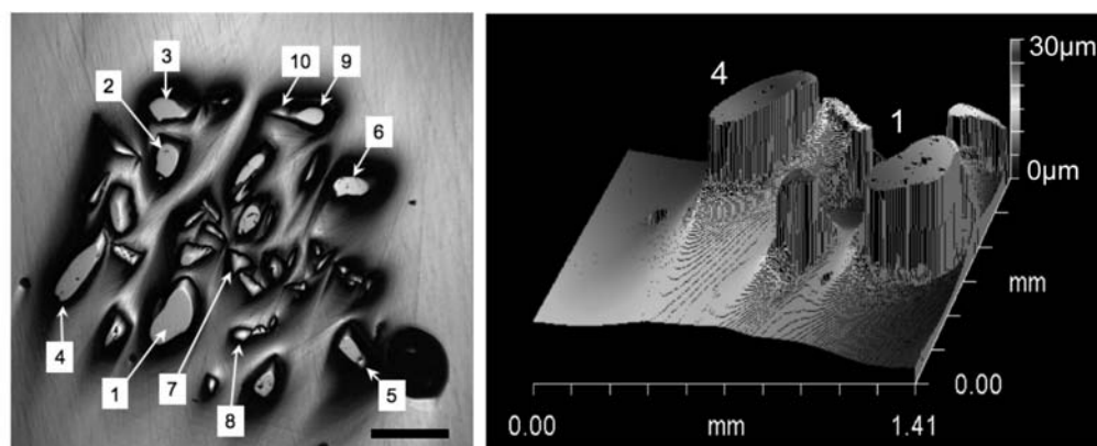
*FIG. 2-12. Zircon grains cast in epoxy showing smooth flat tops and \sim 30 micrometres of relief due to polishing. Left: Zircon grains in reflected light. (Scale = 500 \mu\text{m} ). Right: Polishing relief measured by white light profilometer. Grains 1 and 4 are the same in both images (from Kita et al. 2009).
