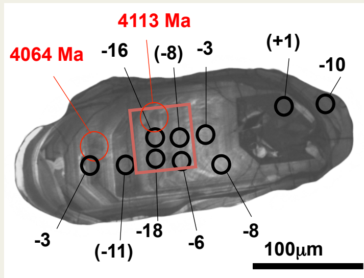
\delta^7\text{Li} correlates with CL domain
