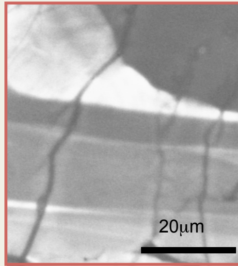
\delta^7\text{Li} correlates with CL domain
