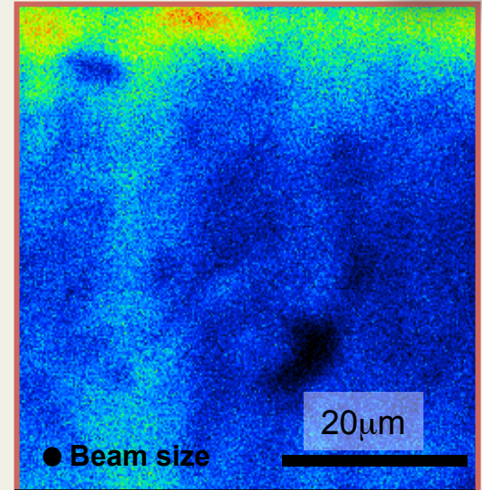
Li concentration correlates with CL domain
