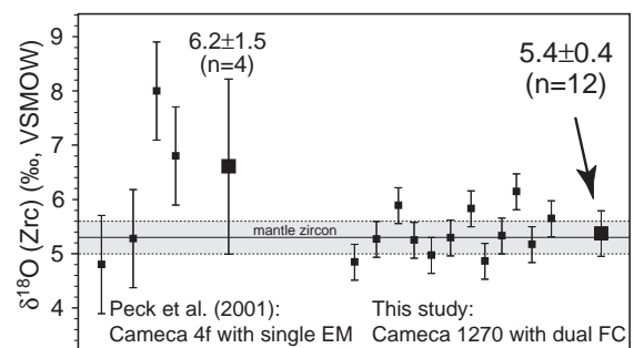
Fig. 5. Comparison of \delta^{18}\text{O} values for zircon W74/2-36 analyzed by multi-collector CAMECA ims-1270 ion microprobe (this study) and by single-collector CAMECA ims-4f [3]. For both groups, the smaller symbols are individual analyses. The larger symbol after each group is the group average. Error bars for individual analyses are the external precision of the standard from the session (1 S.D.). Error bars for group averages are external precision of the individual analyses (1 S.D.). EM=electron multiplier, FC=Faraday cup. See text for discussion.
