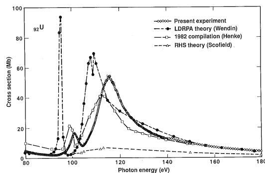
Fig. 2. Experimental photoabsorption cross section for uranium in the region of the 5d-5f resonance compared with theoretical and compiled results. See text for details of the latter curves.
