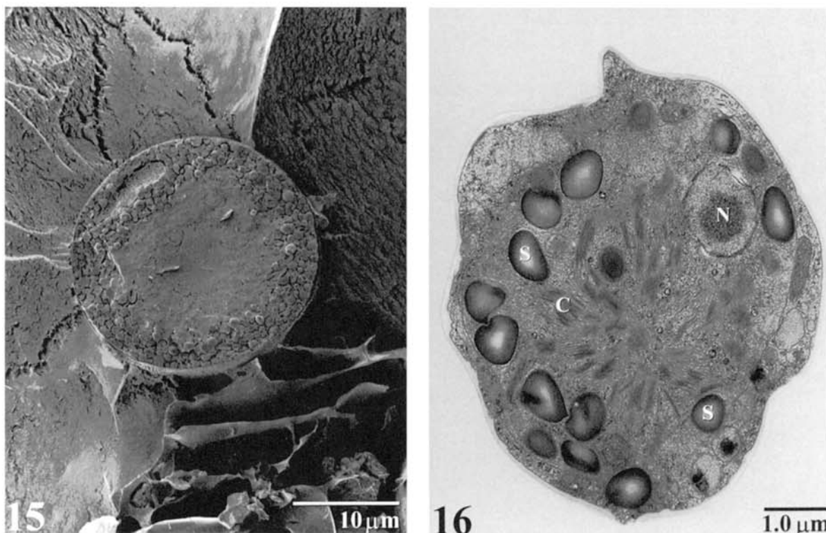
Figure 15. Fractured and etched surface of melting snow illustrating a single cell believed to be a green alga causing the “red snow” phenomenon.
