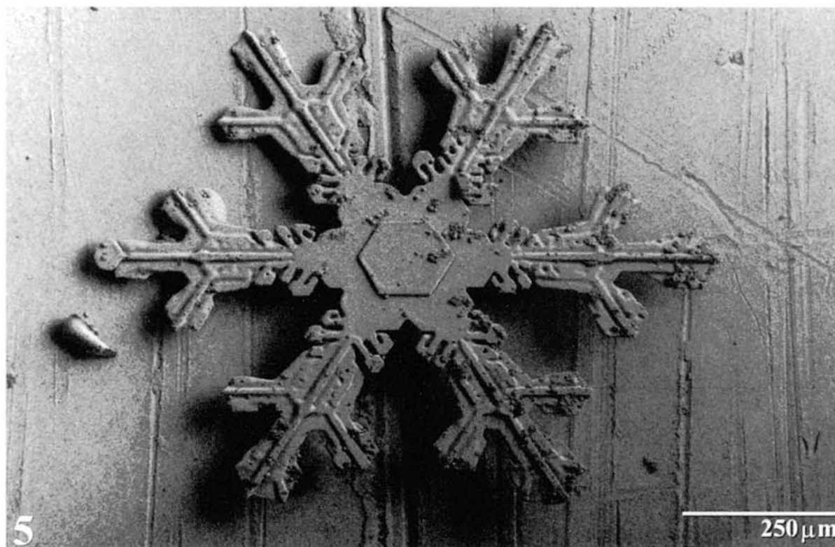
Figure 5. A hexagonal dendrite having a central hexagonal plate. The arms of the dendrite are branched and contain pronounced ridges and small depressions. Sampled at -11^\circ\text{C} air temperature.
