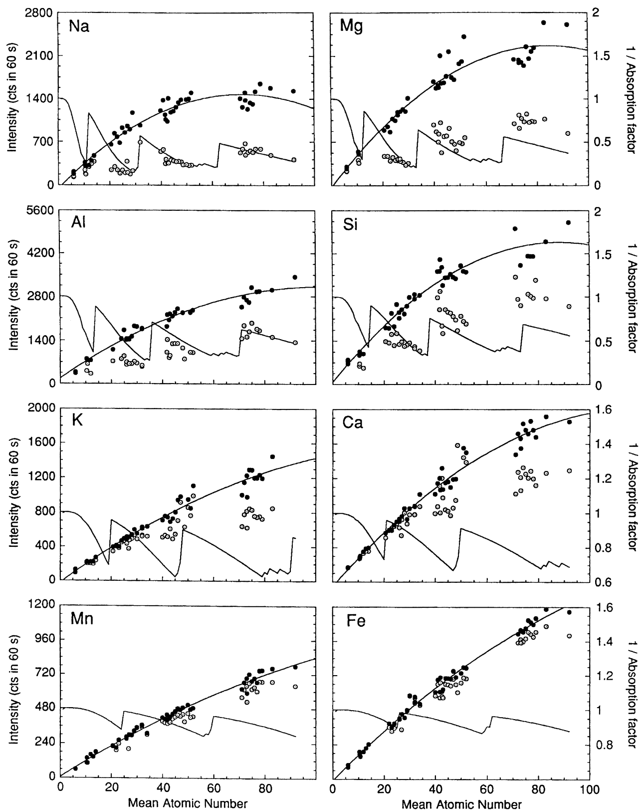
Figure 2. Mean atomic number background data for metals, oxides, and simple binary compounds. Open circles represent the uncorrected intensities for each line measured (Ti and Cr are not shown), closed symbols represent the intensities corrected for continuum absorption as described in the text. The solid line represents the second-order polynomial best-fit to those data. The inverse of the absorption factor (solid line) shows the expected trend of the background data (without the increase in the Bremsstrahlung with increasing atomic number). For Na, Mg, Al, and Si the absorption of the continuum by the various materials can be seen in the uncorrected data.
