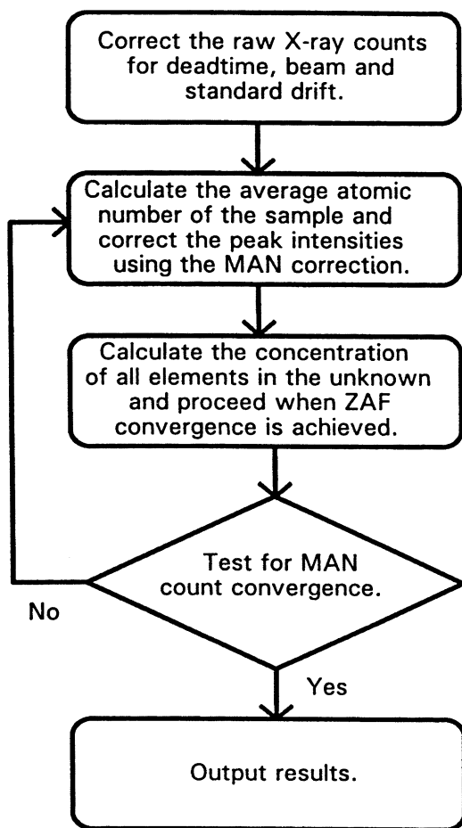
Figure 1. Flow diagram of the MAN background correction presented in this study.
