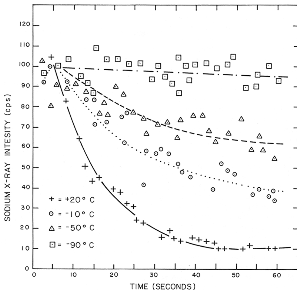
Fig. 3. The effect of sample temperature on sodium-loss from a rhyolitic glass (KN-18) during electron bombardment. Cryogenic cooling of the sample mount to -90^{\circ}\text{C} suppresses alkali diffusion in the glass and enables direct quantitative analysis.
