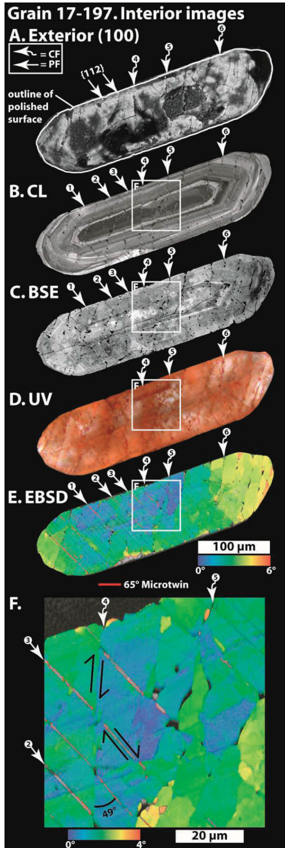
FIGURE 7. Internal images of grain 17-197. (a) Exterior image of the face exposed in the polished section. The white outline shows the location of the polished section. (b) CL image showing oscillatory zoning that is offset in a dextral sense by \{112\} PFs. Curvilinear fractures in an approximately conjugate ( 49^\circ ) orientation to \{112\} are also visible. (c) BSE image showing one orientation of \{112\} PFs and one orientation of curvilinear fractures in approximately conjugate \{112\} orientation. (d) Incident UV light image. The host zircon is largely translucent and PFs in \{112\} are not visible. Curvilinear fractures in sub- \{112\} orientation show distinctly dark zones, indicating they are filled with material that is not zircon. (e) A combined band contrast, local misorientation and grain boundary EBSD map. (f) Higher resolution EBSD map showing \{112\} microtwins offset by curvilinear fractures, 65^\circ grain boundaries are colored red, the gray material within the grain boundaries is in the twinned orientation.
