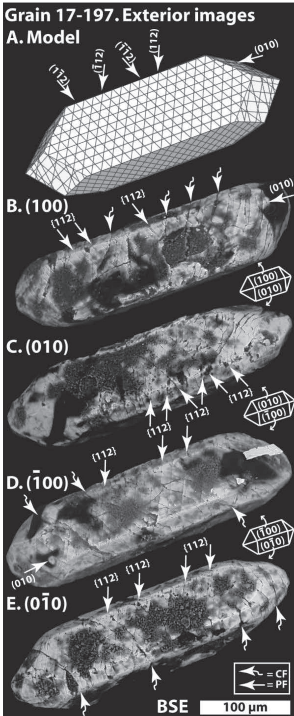
FIGURE 6. External images of detrital shocked zircon grain 17-197 from the center of the Vredefort Dome. (a) Model of a zircon {100} prism with {111} pyramid. The model features four orientations of {112} PFs at 10 μm spacing. (b–e) Exterior BSE images of grain 17-197. Straight arrows indicate PF orientations, curved arrows indicate curvilinear fractures. See enlarged images in Appendix 1 1 .
