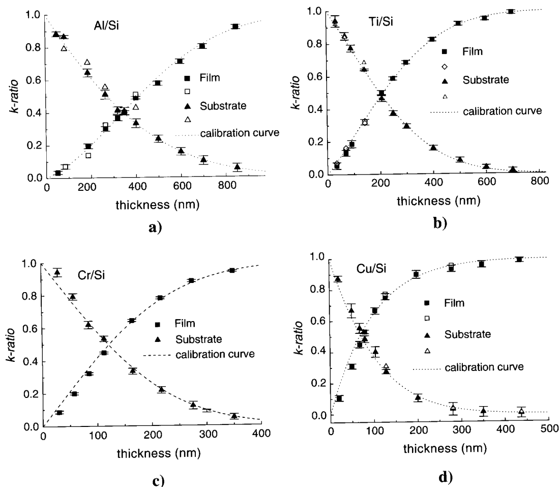
Figure 3. Plots of k -ratio vs thickness with results from experiment and MC simulations for (a) Al/Si, (b) Ti/Si, (c) Cr/Si (only simulations) and (d) Cu/Si films. Open symbols are related to experimental results and solid symbols represent results from Monte Carlo simulations for film and substrate material. The calibration curve, represented by dots, was fitted using Eqn (6). Electron beam energy was 12 keV for these results.
