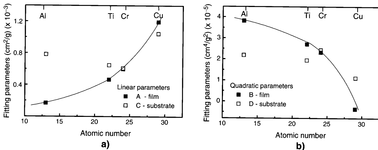
Figure 5. Plots of (a) linear and (b) quadratic fitting parameters against the atomic number from the films characterized through K\alpha x-ray lines and using Eqn (6). Electron beam energy was 12 keV.
