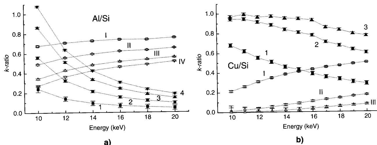
Figure 2. Experimental results for k -ratio versus electron beam energy for (a) Al and (b) Cu films deposited on Si substrate. Numbers 1, 2, 3 and 4 are deposition times in minutes for the film and indicate the measured signal from the films. Numbers I, II, III and IV indicate the corresponding signal measured from the Si substrate.
