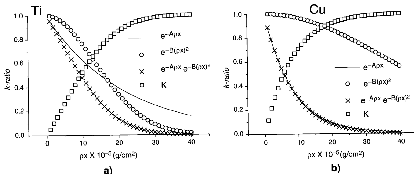
Figure 6. Functional behavior of the linear term and quadratic term in the exponential, and k -ratio of Eqn (6) for (a) Ti/Si and (b) Cu/Si films.
