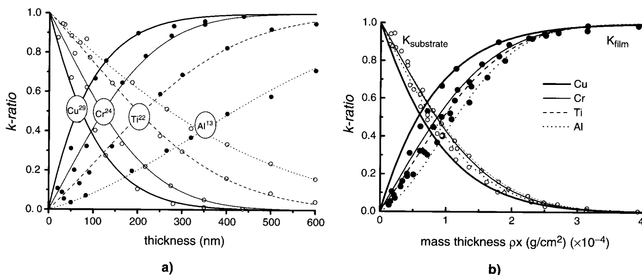
Figure 4. (a) k -ratio vs thickness and (b) k -ratio vs mass thickness with results from MC simulations for Al/Si, Ti/Si, Cr/Si and Cu/Si films and substrate. The calibration curves were fitted using Eqn (6). Electron beam energy was 12 keV for these simulations.
