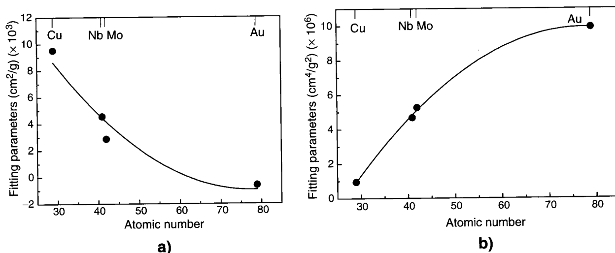
Figure 7. Plots of (a) linear and (b) quadratic fitting parameters against the atomic number from the films characterized through L\alpha x-ray lines and using Eqn (6). Electron beam energy was 12 keV.
