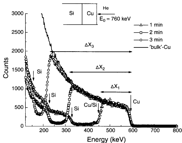
Figure 1. Rutherford backscattering spectra from monoenergetic films of Cu, sputter deposited on Si substrate for different times ( \Delta , 1 min; \square , 2 min; \circ , 3 min; solid line, bulk Cu) \Delta X_i represents the film thickness. Vertical arrows indicate the edge positions at the film surface, film/substrate interface and bulk material.
