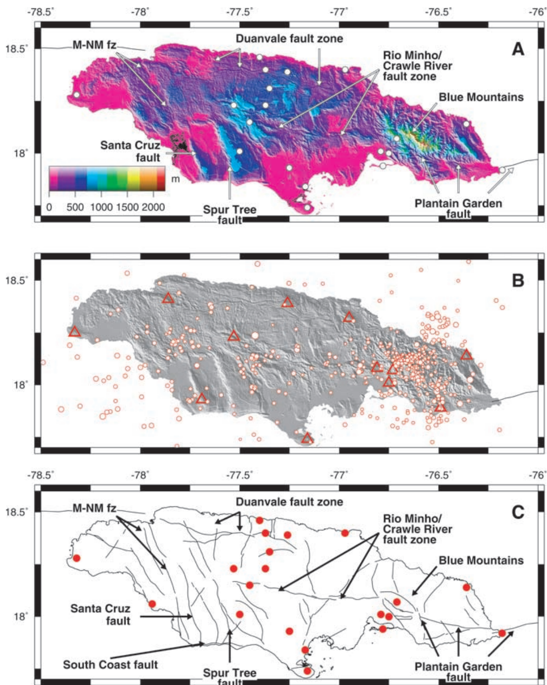
Figure 3. (a) Fault and GPS station locations overlaid on 90-m Space Shuttle Topographic Radar Mission (SRTM) topography illuminated from the southwest. M-NM fz is the Montpelier-New Marker fault zone. (b) The Jamaica Seismograph Network (triangles) and microearthquakes detected by four or more JSN stations for the period 1998–2004 (circles). Only earthquakes with magnitudes equal to or greater than 2.0 are shown, representing the average detection threshold for JSN. Epicentres also include the magnitude 5.1 earthquake of 2005 13 June in central Jamaica. Symbols are scaled to earthquake magnitudes. (c) Locations of GPS stations (red) and potentially active major faults.
