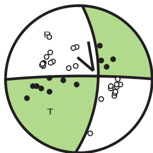
10/04/2017 02h 13mn 19s ML = 4.1 ( 3, 61, 6 )
