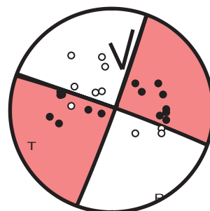
11/04/2017 07h 50mn 36s ML = 2.8 ( 20, 87, 4 )
