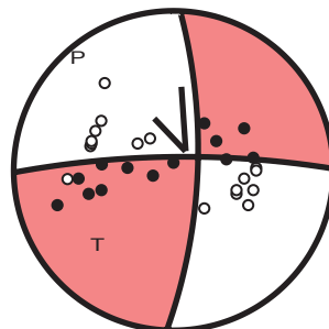
11/04/2017 00h 22mn 06s ML = 3.2 ( 2, 73, 10 )
