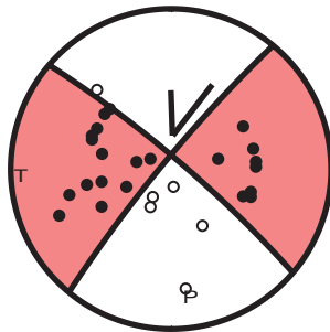
23/04/2017 15h 52mn 52s ML = 3.4 ( 220, 84, -8 )
