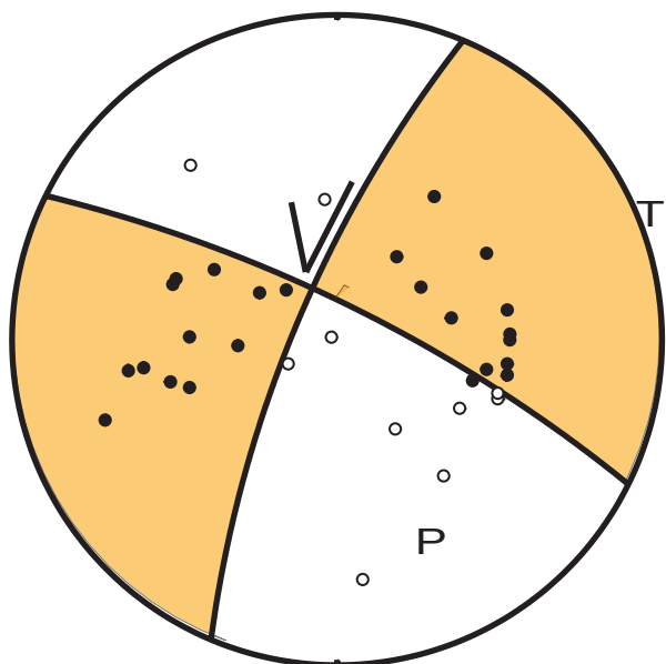
10/04/2017 23h 53mn 55s ( 203, 75, -13 )
