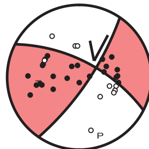
11/04/2017 00h 30mn 37s ML = 3.7 ( 34, 76, 27 )
