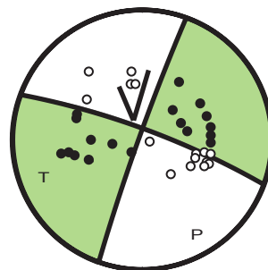
10/04/2017 23h 52mn 57s ML = 4.3 ( 200, 87, -9 )
