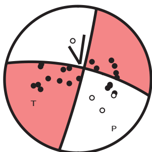
11/04/2017 02h 23mn 24s ML = 3.2 ( 15, 85, 19 )
