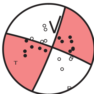
11/04/2017 03h 53mn 11s ML = 2.8 ( 21, 84, 8 )
