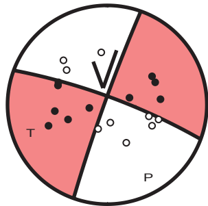
11/04/2017 09h 19mn 28s ML = 2.4 ( 200, 87, -9 )
