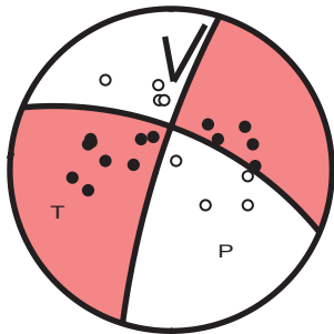
11/04/2017 09h 21mn 42s ML = 2.7 ( 198, 80, -29 )
