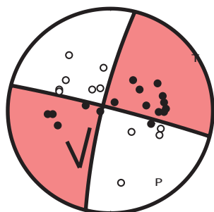
11/04/2017 01h 16mn 32s ML = 3.2 ( 194, 81, -4 )
