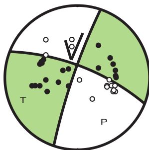
10/04/2017 22h 21mn 45s ML = 3.6 ( 199, 83, -19 )
