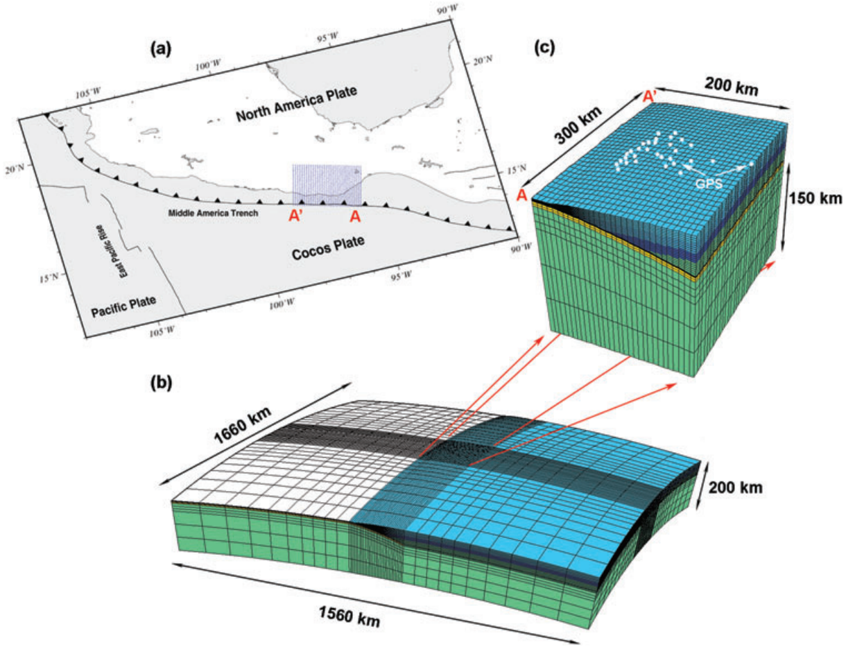
Figure 7. (a) Study area and 3-D finite element mesh. The mesh is built assuming a spherical Earth. (b) Regional mesh with lower and lateral boundaries far from the study area to avoid modelling artefacts. (c) Mesh of the study area and GPS site locations (white circles).
