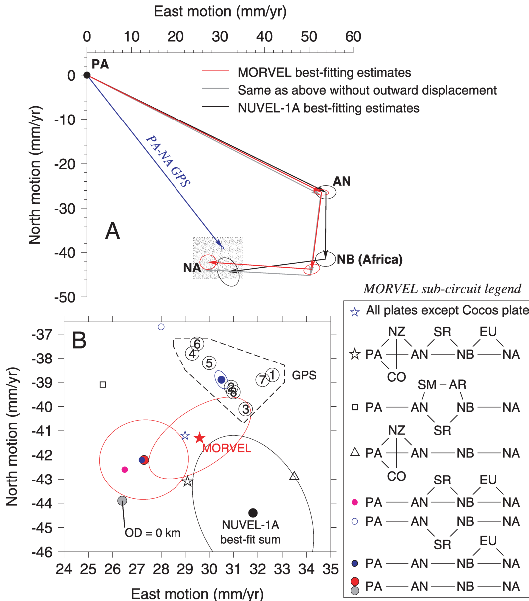
Figure 55. Pacific–North America plate circuit analysis. (a) Linear velocities at 36.0°N, 120.6°W along the San Andreas fault predicted by best-fitting angular velocities determined from the MORVEL data with and without corrections for outward displacement (red and grey, respectively), best-fitting angular velocities determined from the NUVEL-1A data (black), and from GPS (Table 6). No circuit closures are enforced for this plate circuit. Shaded area is enlarged in (b). Plate abbreviations are specified in caption to Fig. 1. (b) North America–Pacific plate motion estimates at 36°N, 120.6°W from different subsets of the MORVEL plate circuits and data (specified in the legend). GPS-based estimates are as follows: 1, DeMets & Dixon (1999); 2, Beavan et al. (2002); 3, Sella et al. (2002); 4, Gonzales-Garcia et al. (2003); 5, Marquez-Azua et al. (2004); 6, Plattner et al. (2007); 7, Kogan & Steblov (2008) and 8, Argus et al. (2010). Blue circle with ellipse is the GPS estimate from this study (Table 6). All ellipses are 2-D, 1 \sigma .
