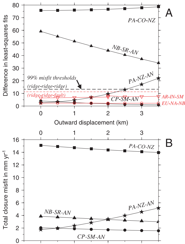
Figure 51. (a) Difference in least-squares fits of best-fitting and closure-enforced angular velocities for three-plate circuits and different assumed values for outward displacement. Black dashed line indicates the value (13.3) above which the difference between the best-fitting and closure-enforced least-squares misfits becomes significant at the 99 per cent confidence level for circuits that meet in ridge–ridge–ridge triple junctions (see text). Red dashed line similarly indicates the 99 per cent confidence threshold (11.3) for ridge–ridge–fault plate circuits (see text). (b) Linear velocities of circuit non-closure at the location of the circuit triple junction, represented by the difference between the linear velocities that are calculated with the best-fitting angular velocity for any one of the three intersecting plate boundaries and the angular velocity that is summed from the best-fitting angular velocities for the other two plate pairs in the circuit (see text). Values are shown only for ridge–ridge–ridge plate circuits since unique velocities of non-closure cannot be determined for ridge–ridge–fault plate circuits.
