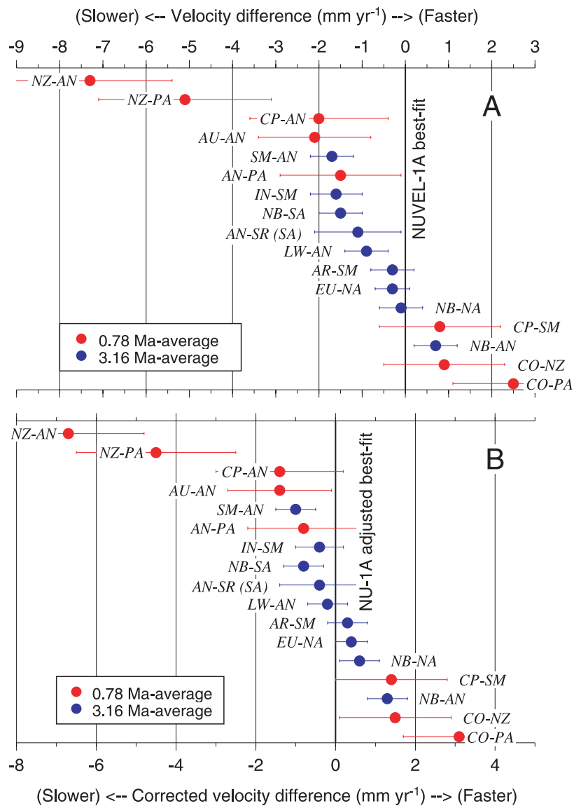
Figure 21. Differences between pure opening-rate components for the MORVEL and NUVEL-1A best-fitting angular velocities (BEAVs) per plate boundary. The pure opening-rate components are the projections of the BEAVs onto an axis that lies 90^\circ from the centroid of the plate boundary along the great circle that includes the pole of rotation. They isolate the uniform component of the spreading rate along the plate boundary from the spreading-rate gradient (Wilson 1993). Differences in both panels are for the MORVEL data relative to the NUVEL-1A data and are expressed in \text{mm yr}^{-1} at the geographic centre of each plate boundary. Panel (a) shows differences per plate pair after applying corrections for outward displacement to the MORVEL but not the NUVEL-1A estimates. Panel (b) shows differences after corrections for outward displacement are applied to both the MORVEL and NUVEL-1A estimates. Standard errors are derived from linear propagation of the formal uncertainties in the MORVEL and NUVEL-1A opening-rate component angles and also incorporate an additional angular uncertainty for an assumed \pm 1 km uncertainty in the magnitude of outward displacement.
