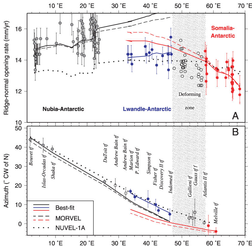
Figure 30. Southwest Indian Ridge spreading rates (a) and transform fault azimuths (b) and rates and directions determined with angular velocities that describe Nubia–Antarctic, Lwandle–Antarctic and Somalia–Antarctic plate motions. Dotted line shows motion determined with the NUVEL-1A Africa–Antarctic angular velocity. All data uncertainties are 1\sigma .
