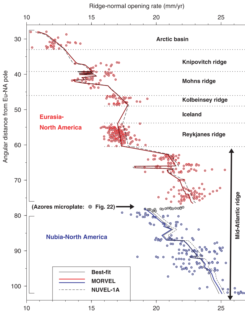
Figure 19. Arctic and north Atlantic basin spreading rates north of 14°N and rates calculated from best-fitting, MORVEL and NUVEL-1A angular velocities. All opening rates in this and later figures have been corrected for outward displacement. Spreading rate uncertainties are omitted for clarity. Fits to directions of motion for Nubia–Eurasia–North America plate circuit are shown in Fig. 20. Additional information about Azores microplate kinematics is given in Fig. 22.
