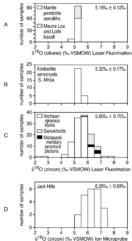
Figure 2. Histograms of \delta^{18}\text{O} . A: Olivine from mantle xenoliths (Matté et al., 1994) and Hawaiian basalts (Eiler et al., 1997). B: Zircon xenocrysts from kimberlites in South Africa (Valley et al., 1998). C: Zircons from igneous rocks of Superior province, Canada (King et al., 1998). D: Ion microprobe analyses of single zircons from Jack Hills, Western Australia (Peck et al., 2001). Superior province histogram (C) peaks at mantle \delta^{18}\text{O} value with tail toward higher values. Jack Hills zircons (D) are higher in \delta^{18}\text{O} than mantle. VSMOW is Vienna standard mean ocean water.
