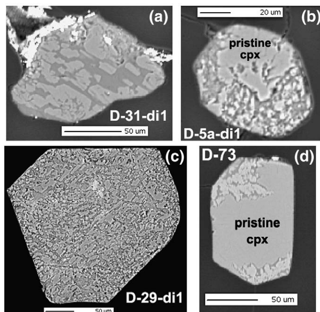
Fig. 7. Back-scattered electron (BSE) images of clinopyroxene inclusions exhibiting spongy textures of secondary alteration in UD-111/02 diamonds. a, b, and d are inclusions exposed on a polished surface. The bright materials in these images are Au left in cracks and depressions from the SIMS study. c is an inclusion extracted from diamond D-29. This inclusion was mounted in epoxy and polished for EMP study.
