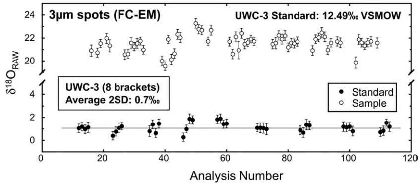
Fig. 5. Optimized reproducibility of SIMS analyses of \delta^{18}\text{O} for UWC-3 calcite standard during a session with a 3\ \mu\text{m} diameter primary beam spot (uncorrected raw data). Data are from Kozdon et al. (2009) who report oxygen isotope zoning in single foram tests. The oxygen isotope analyses were performed using multicollection FC-EM mode. The primary \text{Cs}^+ and secondary ^{16}\text{O}^- ion intensities were \sim 20\text{pA} and 2 \times 10^7 cps, respectively. The integration time was 800 s. A total of 94 analyses were made within 48 h including 36 standard analyses. Filled symbols are UWC-3 analyses and open symbols are analyses of foram samples. The EM high voltage was adjusted before the third of four standard analyses. The average of 2SD of bracketing standard analyses is 0.7‰, while the average internal precision is \sim 0.4\% (2SE), which is consistent with the counting statistics (i.e., total \sim 3 \times 10^7 counts of ^{18}\text{O} in a single analysis).
