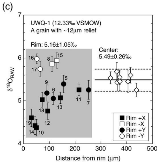
Fig. 11. SIMS oxygen isotope analyses of the center and rim from a quartz standard grain UWQ-1, cast in epoxy with moderate polishing relief (~12 μm). (a, b) Surface topography of a single grain measured using a profilometer. The field of view is 1.4 mm × 1.0 mm. The maximum height difference is 12 μm. The X and Y-axes of the SIMS analyses are shown as white arrows. Numbers in (a) indicate the sequence of analyses. (c) The \delta^{18}\text{O}_{\text{RAW}} values from the rim of the grain show false isotope profile. Data are shown as a distance from the rim. The \delta^{18}\text{O}_{\text{RAW}} values and XY coordinates of individual spots are listed in Table A3. Open diamonds are data from the center of the grain (#1–4, and #20–23) that bracket the rim analyses. Open circles, filled circles, open squares and filled squares are data from rim of the grain towards –Y, +Y, –X, and +X directions, respectively. Numbers next to data symbols are same as in (a). The solid line and dashed lines are the average and 2SD of the data from the center of the grain. Most of rim data within 100 μm from the edge of the grain are outside of 2SD defined by the data from the center. Large negative deviations in \delta^{18}\text{O}_{\text{RAW}} values from those of data at the center are seen from spots located at +X and +Y positions (filled symbols), while data from opposite sides (–X and –Y, open symbols) show slightly higher \delta^{18}\text{O}_{\text{RAW}} values than the center.
