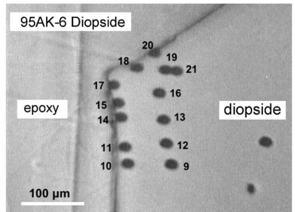
Fig. 12. Optimized SIMS oxygen isotope analyses of the rim of diopside standard (95AK-6) showing minimal polishing relief (<1 μm). (a) The data from edge (open symbols, <20 μm from the edge) and inside (filled symbols, ~100 μm from the edge) are indistinguishable within analytical uncertainty (difference between inside and edge: 0.05 \pm 0.12\text{‰} , 2SE). (b) Reflected light image of the grain boundary between diopside and epoxy resin. The positions of the SIMS pits are shown with the analysis number; data are in Table A4.
