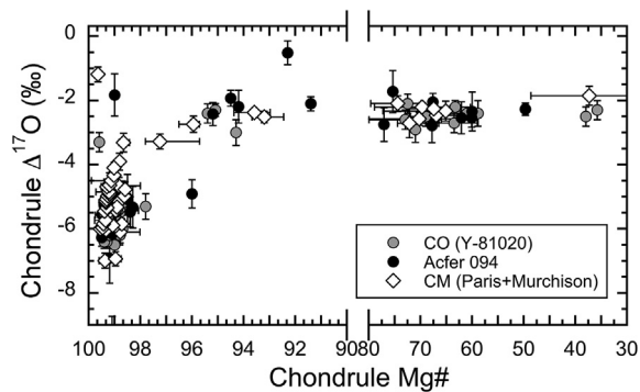
Fig. 8. \Delta^{17}\text{O} values vs. Mg#s of individual host chondrules in CM (open diamonds; Chaumard et al., 2018; this work), CO (grey circles; Tenner et al., 2013), and Acfer 094 (black circles; Ushikubo et al., 2012) chondrites. Chondrule Mg# uncertainties correspond to the range of measured values, while uncertainties in \Delta^{17}\text{O} are the propagated 2SE.
