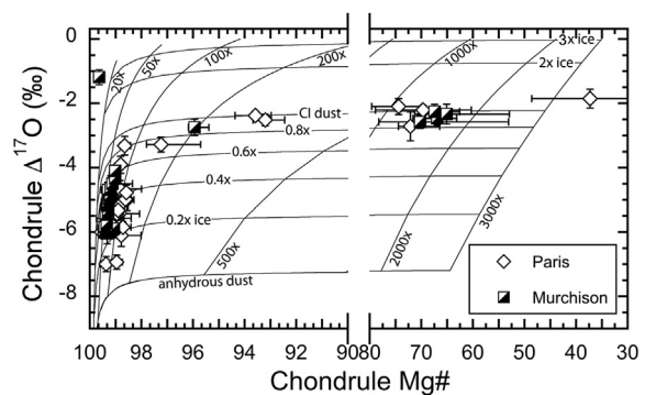
Fig. 9. \Delta^{17}\text{O} values of individual host chondrules in the CM chondrites Paris (this work) and Murchison (Chaumard et al., 2018) and Mg#s superimposed by oxygen isotope mixing curves of constant dust enrichment and ice enhancement from Tenner et al. (2015) and Hertwig et al. (2018). In this model, the anhydrous silicate dust, Solar gas, water ice, and organics in the dust are considered to have \Delta^{17}\text{O} values of -8\text{‰} , -28.4\text{‰} , +2.0\text{‰} , and +11.3\text{‰} , respectively (Hertwig et al., 2018). Chondrule Mg# uncertainties correspond to the range of measured values, while uncertainties in \Delta^{17}\text{O} are the propagated 2SE.
