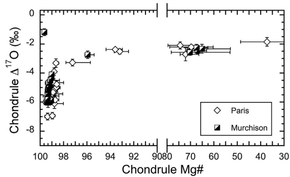
Fig. 7. \Delta^{17}\text{O} values of individual host chondrules in Paris vs. Mg#s (open diamonds). Data from the Murchison CM2 chondrite (black and white squares; Chaumard et al., 2018) are shown for comparison. Chondrule Mg# uncertainties correspond to the range of measured values, while uncertainties in \Delta^{17}\text{O} are the propagated 2SE.
