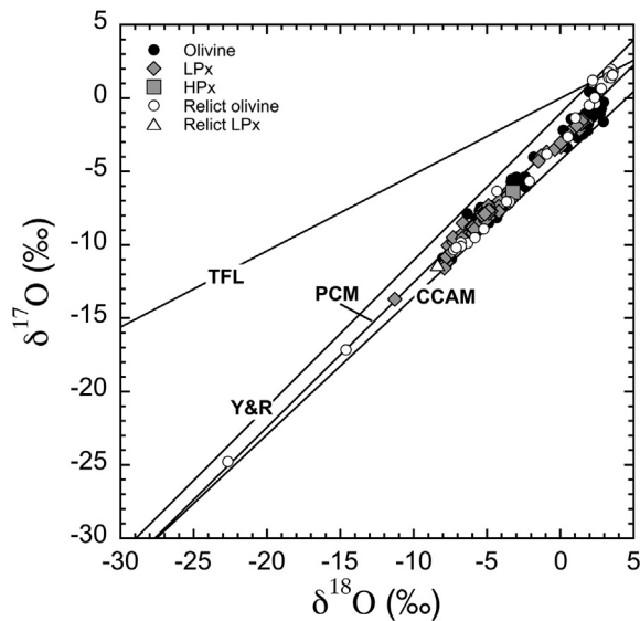
Fig. 5. Oxygen three-isotope diagram of individual spot analyses of olivine, Low-Ca pyroxene (Lpx), high-Ca pyroxene (Hpx), and relict grains in chondrules in Paris. Error bars, corresponding to the spot-to-spot reproducibility (2SD), are smaller than the symbol sizes. The CCAM (carbonaceous chondrite anhydrous mineral; Clayton et al., 1977), Y&R (Young and Russell, 1998), and PCM (primitive chondrule minerals; Ushikubo et al., 2012) lines are shown for reference. The terrestrial fractionation line (TFL) is also shown.
