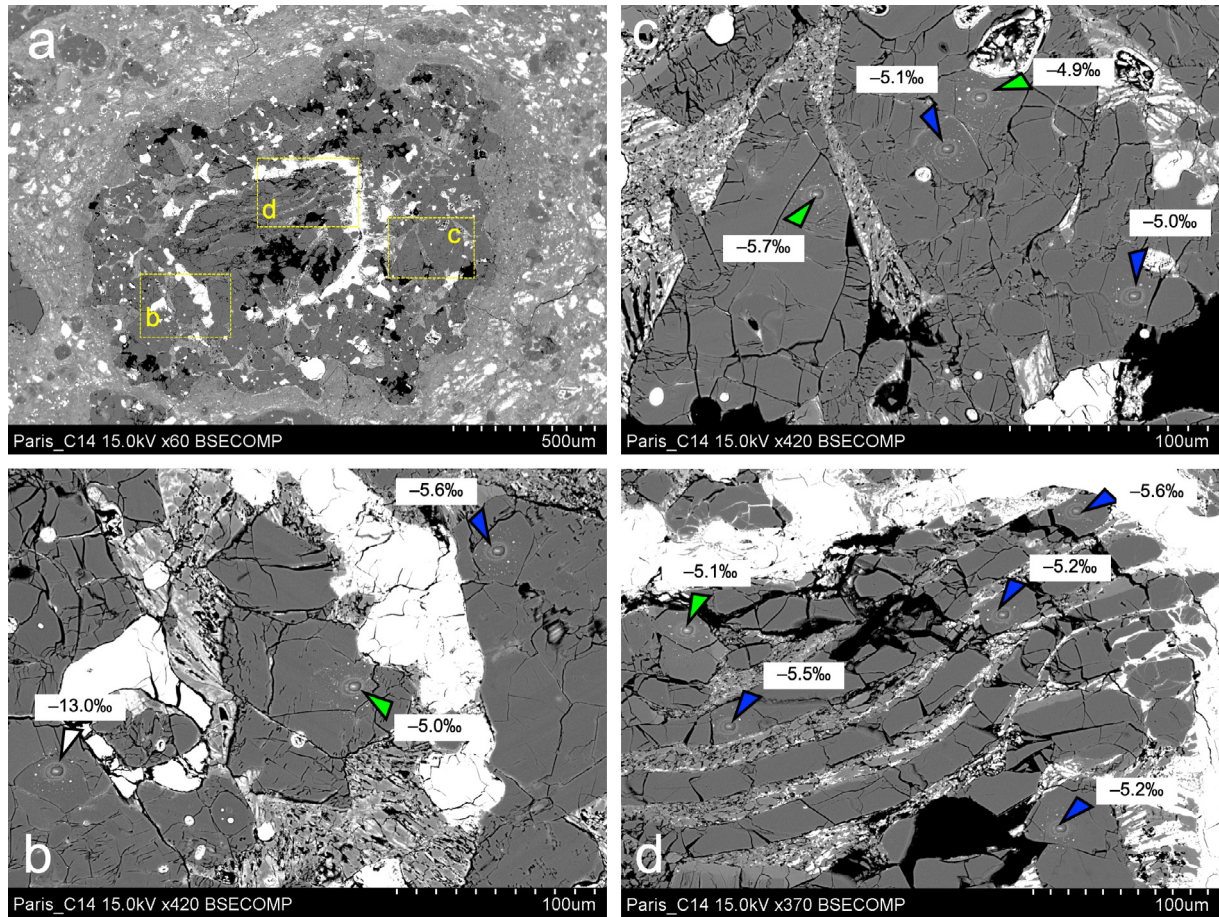
Fig. 3. BSE images of the type I chondrule C14 analyzed in Paris. (a) the entire image of the chondrule, (b-d) expanded images. SIMS oxygen three-isotope analysis points are shown by the vertex of the triangles, color-coded for mineral phases (olivine: blue, relict olivine: white, low-Ca pyroxene: green). \Delta^{17}\text{O} values of individual analyses are indicated. (For interpretation of the reference to color in this figure legend, the reader is referred to the web version of this article).
