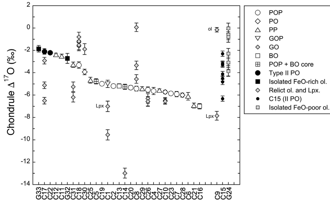
Fig. 6. \Delta^{17}\text{O} values of individual host chondrules and isolated olivine grains in Paris. Relict olivine (ol) and low-Ca pyroxene (Lpx) grains are shown together. Data are sorted according to the host \Delta^{17}\text{O} values. Chondrule C9 (GO) contains homogeneously ^{16}\text{O} -poor olivine, which is likely relict. A single analysis of pyroxene would represent melt oxygen isotope ratios that show lower \Delta^{17}\text{O} compared to other host chondrule values. For the heterogeneous chondrule C15 (II PO) and isolated Fe-poor olivine grain G24, individual analyses are shown. Error bars represents the propagated uncertainties for host chondrules and olivine in C9, and external reproducibility of individual analyses for relict grains, pyroxene in C9, and all data in C15 and G24.
