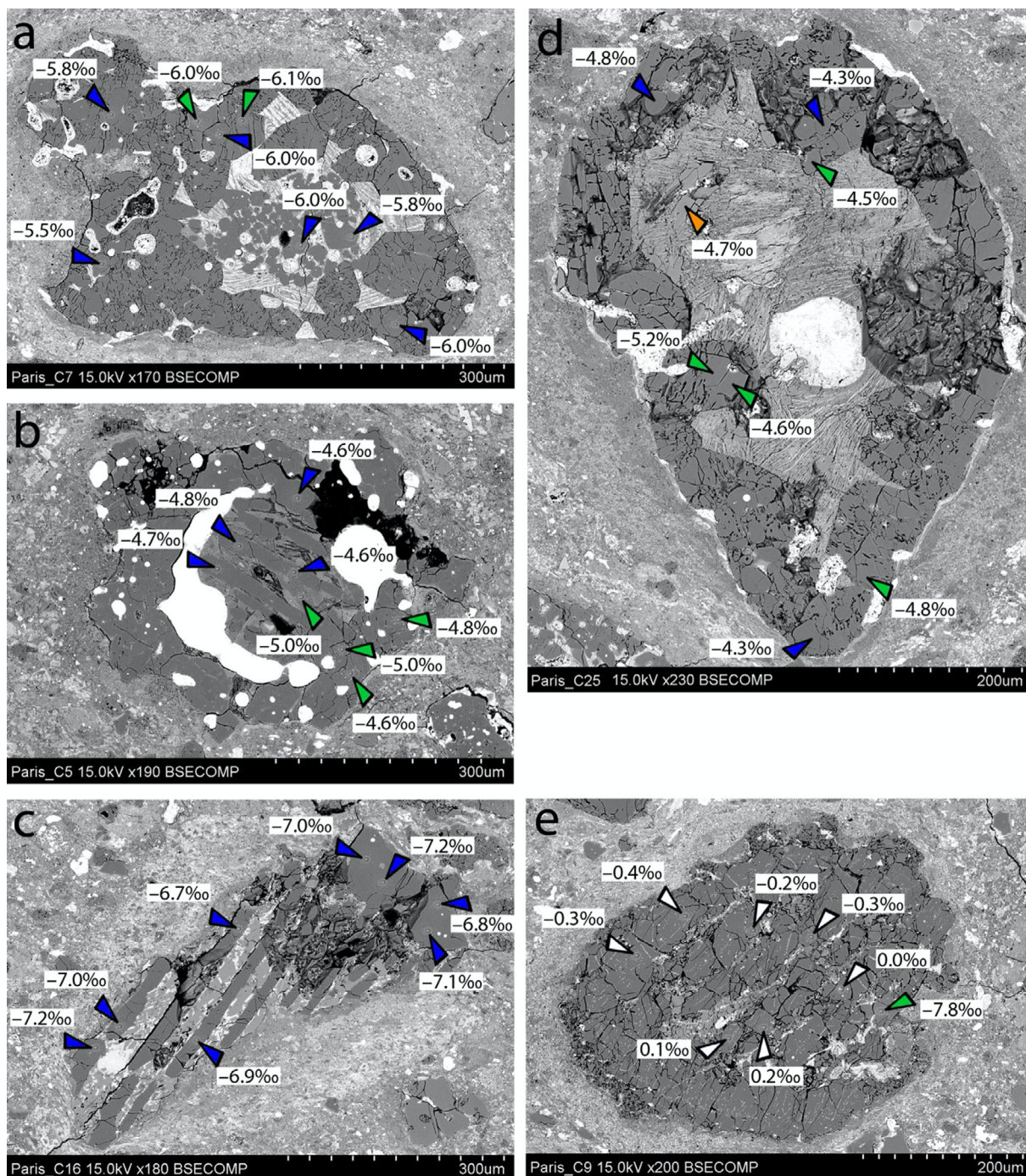
Fig. 2. BSE images of type I chondrules analyzed in Paris displaying various textures. (a) C7: POP, (b) C5: POP + BO core, (c) C16: BO fragment, (d) C25: PP, and (e) C9: GO. SIMS oxygen three-isotope analysis points are shown by the vertex of the triangles, color-coded for mineral phases (olivine: blue, relict olivine: white, low-Ca pyroxene: green, high-Ca pyroxene: orange). \Delta^{17}\text{O} values of individual analyses are indicated. (For interpretation of the references to color in this figure legend, the reader is referred to the web version of this article).
