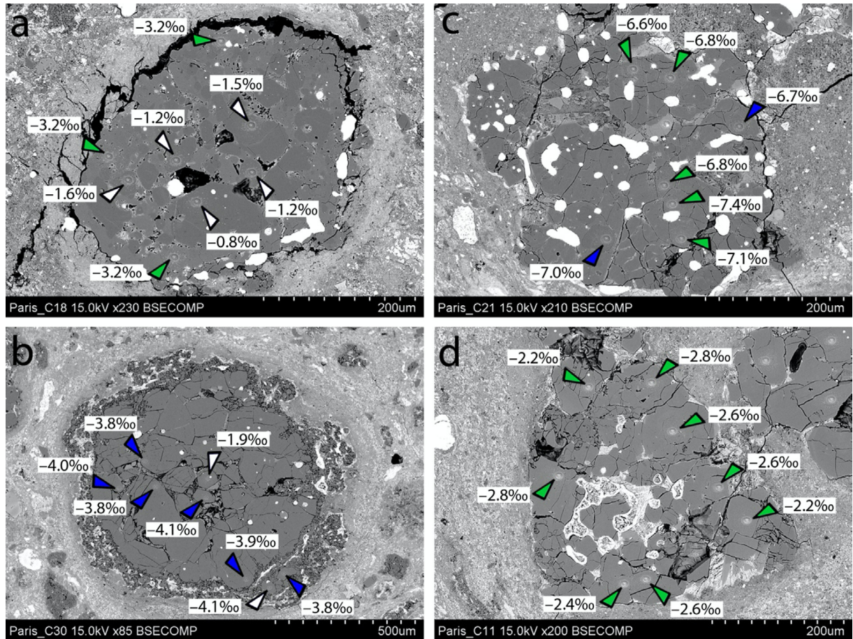
Fig. 1. BSE images of type I porphyritic chondrules analyzed in Paris. (a) C18: POP, (b) C30: PO, (c) C21: PP, and (d) C11: PP. SIMS oxygen three-isotope analysis points are shown by the vertex of the triangles, color-coded for mineral phases (olivine: blue, relict olivine: white, low-Ca pyroxene: green). \Delta^{17}\text{O} values of individual analyses are indicated. (For interpretation of the references to color in this figure legend, the reader is referred to the web version of this article).
