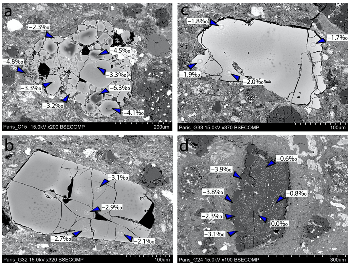
Fig. 4. BSE images of a type II PO chondrule (C15), two isolated Fe-rich olivine grains (G32 and G33), and an isolated Fe-poor olivine grain (G24) analyzed in Paris. (a) C15, (b) G32, (c) G33, (d) G24. SIMS oxygen three-isotope analysis points are shown by the vertex of the triangles, color-coded for olivine (blue). \Delta^{17}\text{O} values of individual analyses are indicated. (For interpretation of the reference to color in this figure legend, the reader is referred to the web version of this article).
