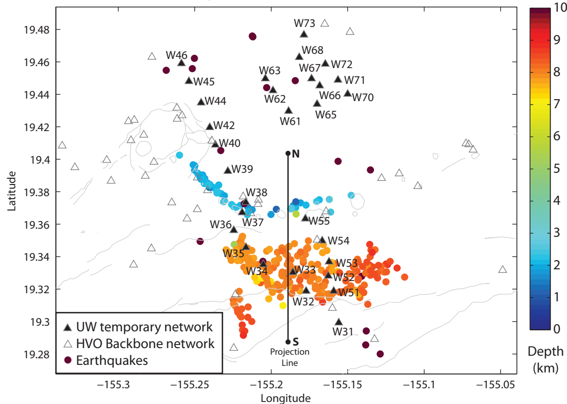
Relocated Earthquakes from Nov. 1999 to June 2000
