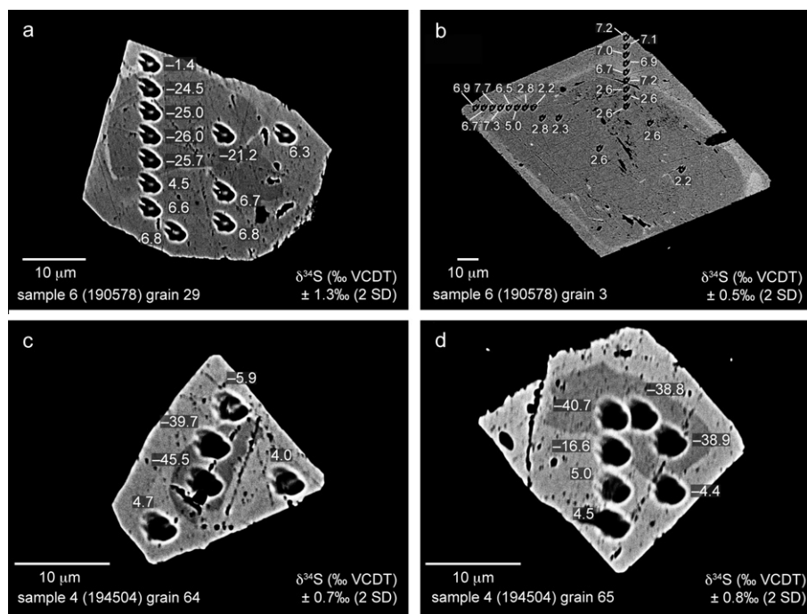
Fig. 5. (a–d) Backscattered electron images of pyrite grains showing analytical pits from WiscSIMS and measured \delta^{34}\text{S} values from the Meteorite Bore Member of the Turee Creek Group, Western Australia. Darker cores and brighter rims are isotopically distinct. Rims have \delta^{34}\text{S} consistent with a hydrothermal origin, whereas cores in a, c and d have low \delta^{34}\text{S} consistent with an origin from microbial sulfate reduction. Analytical pits that straddle core–rim boundaries have intermediate \delta^{34}\text{S} reflecting mixing of distinct zones.
