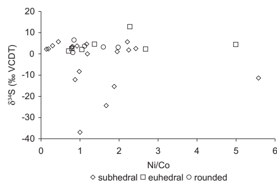
Fig. 11. Sulfur isotope composition vs. Ni/Co in Meteorite Bore Member pyrites with both Ni and Co present above minimum detection limits. Grains are grouped by morphology, and rounded grains are classified as detrital. Grains with \delta^{34}\text{S} indicative of microbial sulfate reduction have \text{Ni/Co} > 0.8 .
