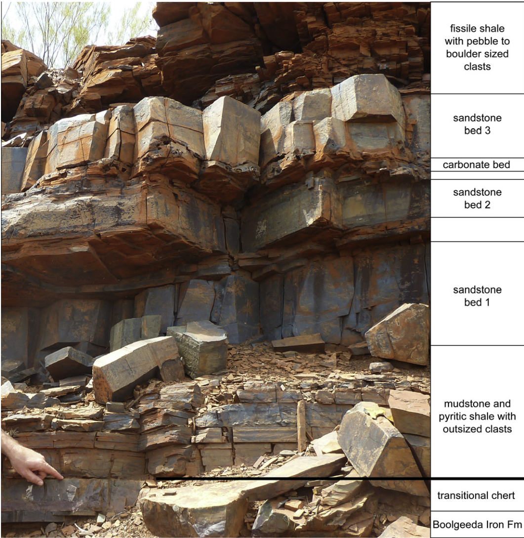
Fig. 2. Exposure of the Meteorite Bore member in outcrop at the Boundary Ridge locality (Fig. 1) with hand for scale. Finger is pointing at the contact between the “transitional chert” and the first siliciclastic unit, representing the onset of glaciomarine sedimentation. This also marks the conformable boundary between the uppermost Hamersley Group (Boolgeeda Iron Fm) and the lowermost Turee Creek Group. Lithologic descriptions are given in the stratigraphic column at right, shown in greater detail in Fig. 3.
