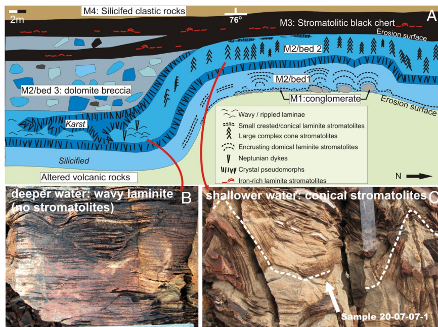
Fig. 4. Stromatolites at the platform margin outcrop on southern Trendall Ridge. (A) Outcrop map showing cross-section view of stratigraphy from underlying altered volcanic rocks up through members 1–3 and part of member 4 of the Strelley Pool Formation. Note the paleotopographic feature on which the stromatolites were deposited: stromatolites only formed on the high side (Right). (B) Wavy laminites deposited in deeper water south of the paleohigh. (C) LCC (conical) stromatolites formed on the paleohigh. The dotted white line traces a single lamina across 2 coniform stromatolites. The sample indicated is shown in Fig. 5. (Scale rule in B and C: 15 cm.) Modified from ref. 32.
