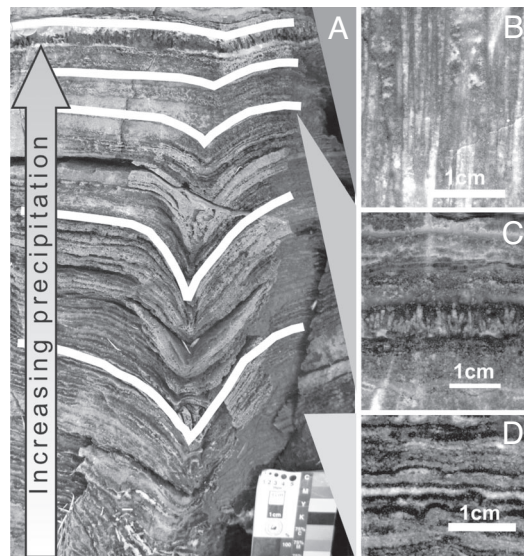
Fig. 3. Images showing the vertical trend in fabrics and parallel change in laminar architecture through the encrusting/domical stromatolites. (A) Outcrop exposure showing part of 2 broad domical stromatolites and the cusped depression in between. The lower strata show irregularly laminated fabrics with inferred clastic textures; laminae thin toward the margins and laminar geometry does not change significantly through successive layers. The abundance of precipitated textures (palisades, acicular crystal pseudomorphs) increases in the upper strata, where laminae maintain thickness laterally and the laminar geometry changes with each successive layer. Consequently, the cusp infills and the domes coalesce. Scale increments on card = 1 cm. (B) Polished slab showing acicular crystal pseudomorphs from strata \approx 30 cm above the top of the photo in A. (C) Polished slab showing palisaded layer among irregular lamination. (D) Polished slab showing irregular lamination with organic layers (black laminae).
