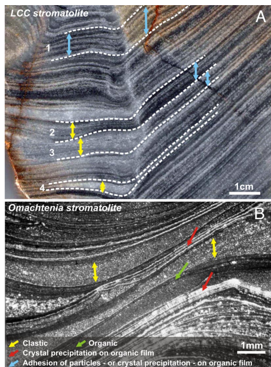
Fig. 5. Sedimentary fabrics of an Early Archean coniform stromatolite and Mesoproterozoic Omachtenia stromatolite. (A) Coniform LCC stromatolite from the Early Archean Strelley Pool Formation. The stromatolite is on the right, and flat-lying intercolumn laminae are on the left. Polished slab showing a cross-section view. Dark laminae are chert-rich, light laminae are dolomite-rich. Dark cross-cutting fractures filled with hematite are the result of recent weathering. Dotted white lines highlight bundles of laminae with different character. Numbers refer to locations discussed in text. (B) Mesoproterozoic O. omachtensis stromatolite from the Uchuro-Maya region, Siberia, showing precipitated and clastic textures with thin organic laminae. Thin section, plane polarized light. Colored arrows on laminae indicate the inferred processes by which those laminae formed.
