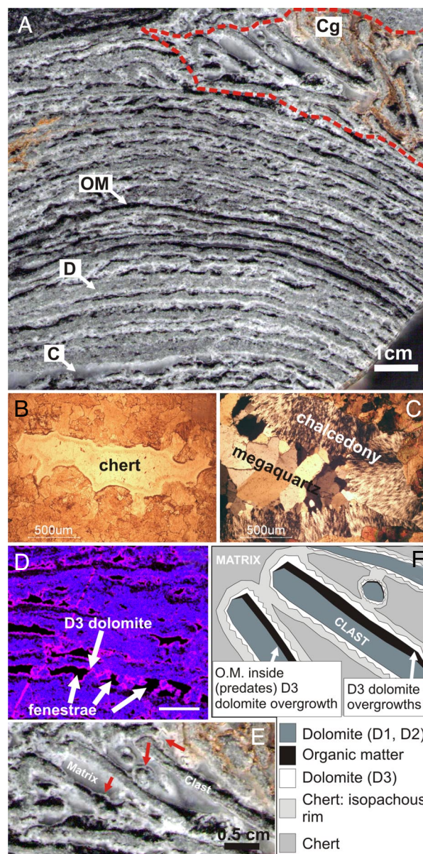
Fig. 1. Encrusting/domical stromatolite fabrics. (A) Polished slab, showing irregularly wrinkly laminar fabric consisting of dolomite (D), chert (C), and organic laminae (OM). Note organic layers on upper sides of flat pebble intraclast conglomerate (Cg, outlined in dotted red line) piled against upper right of stromatolite. (B) Chert-filled fenestra surrounded by D2 dolomite are shown. Transmitted plane polarized light. (C) Detail of cavity fill chert with chalcidony at margins and megaquartz at the center. Transmitted cross polarized light. (D) Composite X-ray fluorescence map of Ca (blue) and Fe (pink). The brighter pink areas highlight the greater Fe content of D3 dolomite compared with D1 and D2 in the surrounding dolomite (blue) laminae. The black areas in the rock fabric represent silica. (Scale bar: 0.5 cm.) (E) Detail of intraclast conglomerate from upper right corner of the sample shown in A. Red arrows point to white rims surrounding the clasts and organic material. The rims consist of D3 dolomite overgrowths (inner) and isopachous chert rims (outer). (F) Schematic illustration of the relationship between clasts, organic deposits, dolomite overgrowths and chert in the intraclast conglomerate shown in E.
