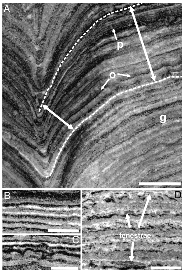
Fig. 2. Fabrics in lower to middle strata of encrusting/domical stromatolites at Anchor Ridge. (A) Polished slab showing edge of domical stromatolite with organic laminae and variable recrystallization. Note laminae become thinner toward margin, as shown by the dotted white lines and large arrows oriented normal to the paleosurface of the stromatolite. As a result, the cusp and dome geometry do not change significantly through successive layers. g, inferred clastic or grainy fabric; p, relict palisades (precipitated) fabric; o, organic laminae. (B) Polished slab showing detail of inferred relict clastic texture with organic laminae (black layers) and dolomite laminae with minor chert (gray layers). (C) Polished slab showing detail of inferred clastic texture with organic laminae (black layers) and incipient domical structures. (D) Polished slab showing detail of irregular laminoid fabric with organic laminae, chert-filled fenestrae and inferred relict grainy texture. (Scale bars: \approx 1 cm.)
