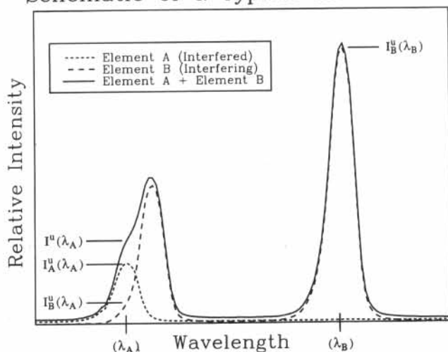
FIGURE 1. Schematic diagram showing a hypothetical spectral interference.
