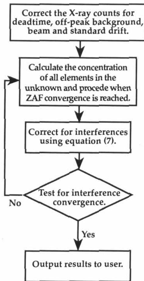
FIGURE 2. Flow diagram of the interference correction presented in this study.
